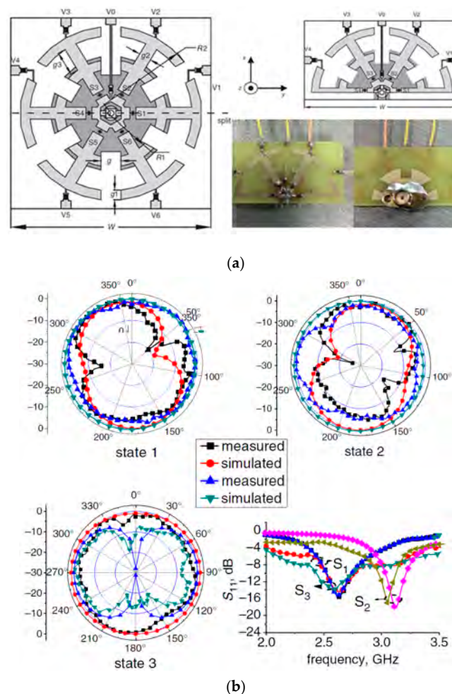
Figure 6. (a) Configuration and (b) performance of the frequency and pattern reconfigurable antenna in [65]. Reproduced with permission from [65], Copyright IEEE, 2015.
